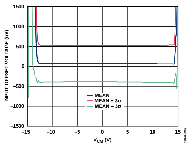
Figure 14. Input Offset Voltage vs. Input Common-Mode Voltage ( V_{CM} ), V_{SY} = \pm 15\text{ V} , R_L = \infty
