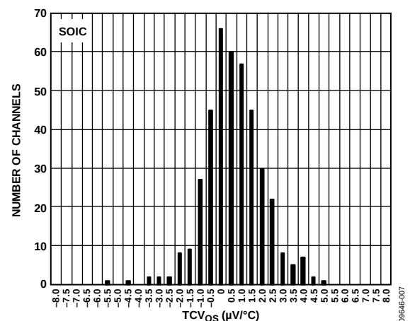
Figure 13. TCV_{OS} Distribution, V_{SY} = \pm 15\text{ V}
