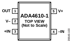
Figure 3. ADA4610-1 Pin Configuration, 5-Lead SOT-23 (RJ Suffix)
