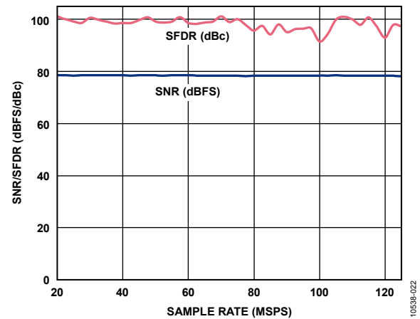
Figure 22. SNR/SFDR vs. Sample Rate, f_{IN} = 9.7 \text{ MHz} , V_{REF} = 1.0 \text{ V}
