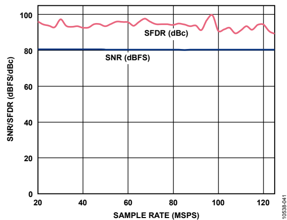
Figure 41. SNR/SFDR vs. Sample Rate, f_{IN} = 9.7 MHz, V_{REF} = 1.3 V
