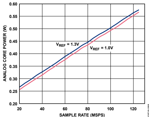
Figure 70. Analog Core Power vs. f_{\text{SAMPLE}} for f_{\text{IN}} = 9.7 \text{ MHz} , Four Channels
