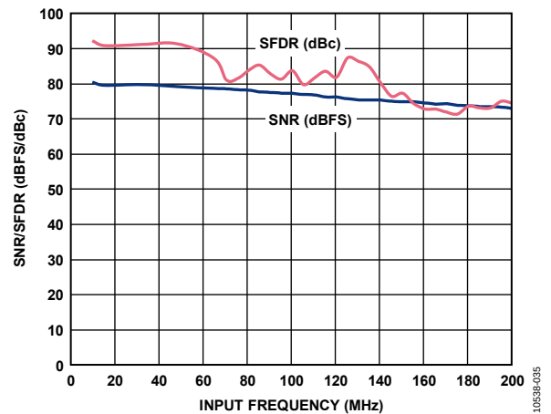
Figure 35. SNR/SFDR vs. f_{IN} , f_{SAMPLE} = 125 MSPS, Clock Divider = 8, V_{REF} = 1.3 V
