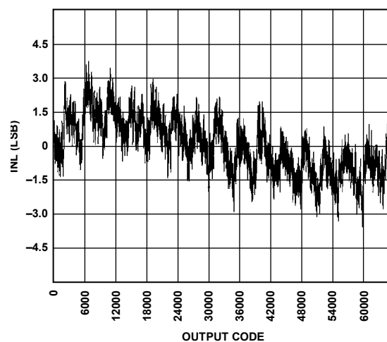
Figure 18. INL, f_{IN} = 9.7 MHz, f_{SAMPLE} = 125 MSPS, V_{REF} = 1.0 V
