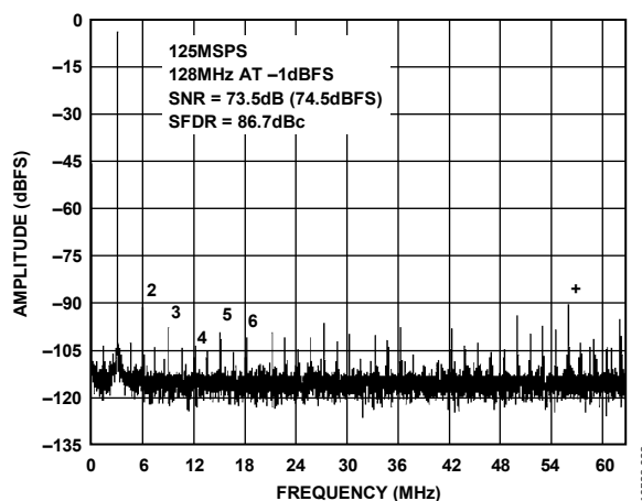
Figure 28. Single-Tone 16k FFT with f_{IN} = 128\text{ MHz} , f_{SAMPLE} = 125\text{ MSPS} , V_{REF} = 1.3\text{ V}
