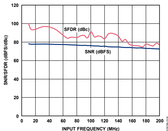
Figure 16. SNR/SFDR vs. f_{IN} , f_{SAMPLE} = 125 MSPS, Clock Divider = 8, V_{REF} = 1.0 V
