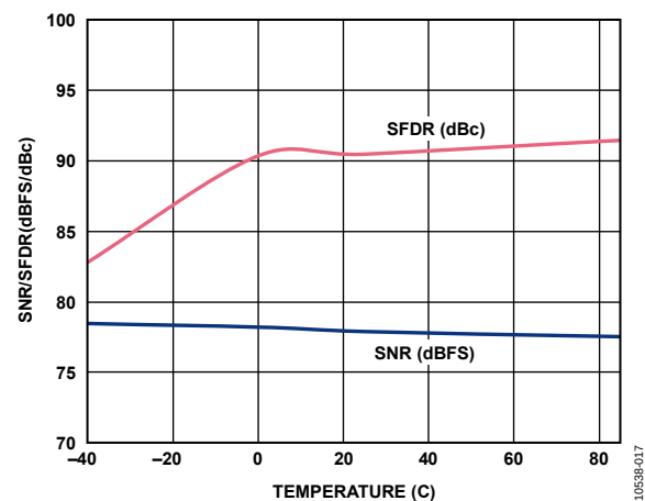
Figure 17. SNR/SFDR vs. Temperature, f_{IN} = 9.7 MHz, f_{SAMPLE} = 125 MSPS, V_{REF} = 1.0 V
