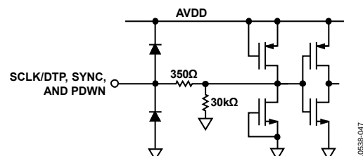
Figure 47. Equivalent SCLK/DTP, SYNC, and PDWN Input Circuit
