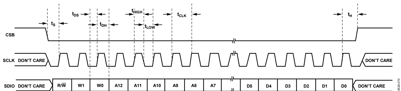
Figure 75. Serial Port Interface Timing Diagram
