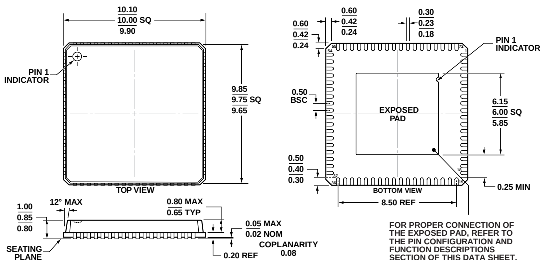
Figure 51. 72-Lead Lead Frame Chip Scale Package [LFCSP_VQ] 10 mm x 10 mm Body, Very Thin Quad (CP-72-7)
