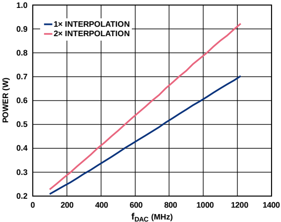
Figure 19. Total Power Consumption vs. f_{DAC} over Interpolation
