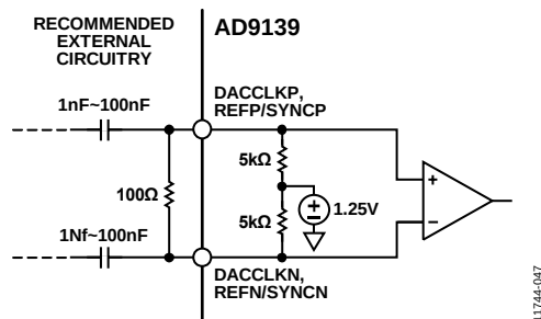
Figure 42. Clock Receiver Input Simplified Equivalent Circuit
