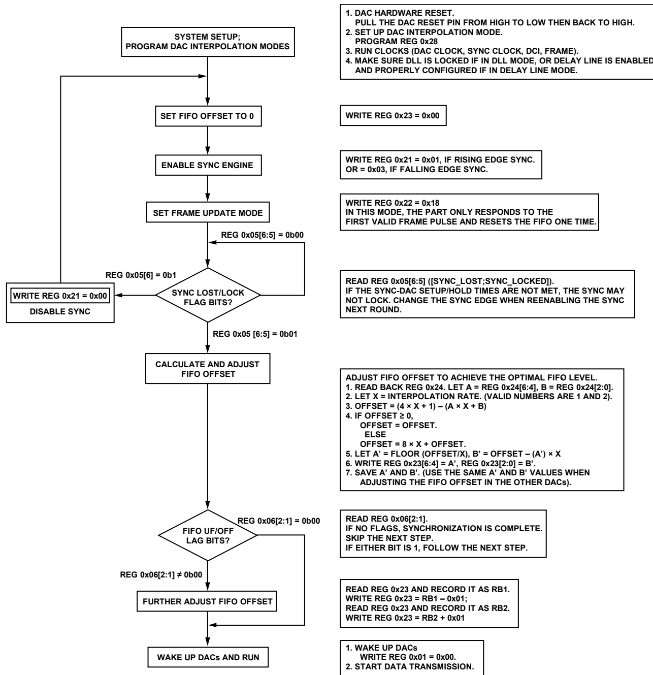
Figure 39. Synchronization Procedure Diagram
