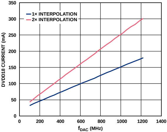
Figure 20. DVDD18 Current vs. f_{DAC} over Interpolation
