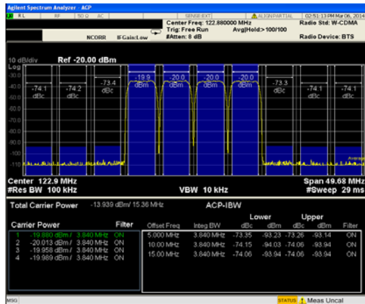
Figure 23. 4C WCDMA ACLR, f_{OUT} = 122 MHz, f_{DAC} = 983 MHz, 2× Interpolation, PLL Frequency = 122 MHz
