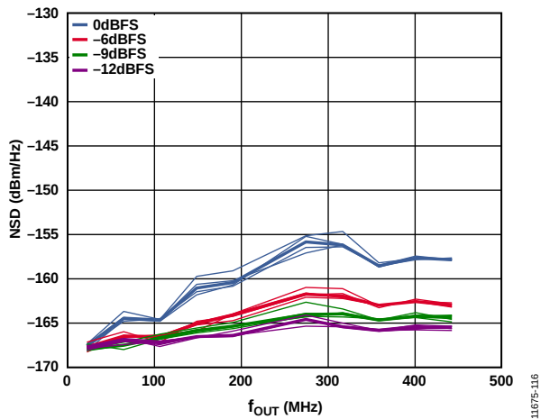
Figure 16. Single-Tone NSD vs. f_{OUT} over Digital Back Off, f_{DAC} = 983 \text{ MHz}
