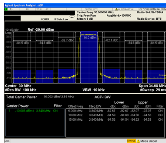
Figure 20. 1C WCDMA ACLR, f_{OUT} = 30 \text{ MHz} , f_{DAC} = 983 \text{ MHz} , 2× Interpolation, PLL Frequency = 122 MHz
