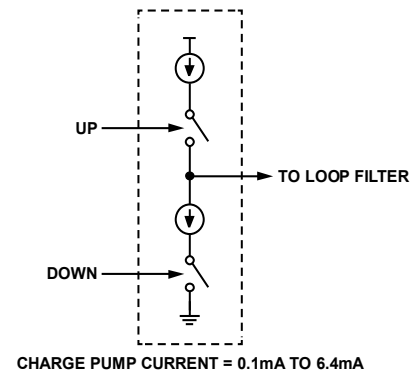
Figure 78. Charge Pump
