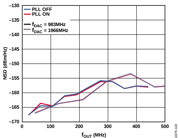
Figure 18. Single-Tone NSD (0 dBFS) vs. f_{OUT} , f_{DAC} = 983 \text{ MHz} and 1966 \text{ MHz} , PLL On and Off
