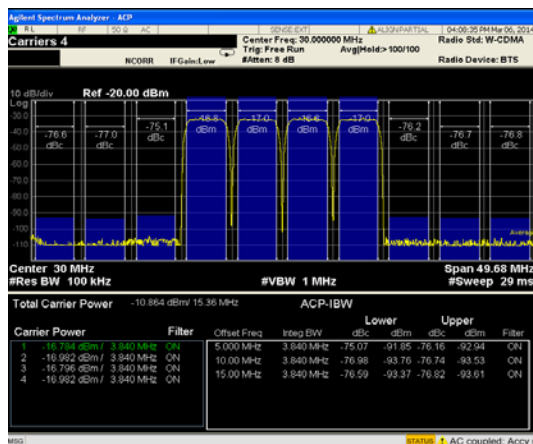
Figure 24. 4C WCDMA ACLR, f_{OUT} = 30 MHz, f_{DAC} = 1966 MHz, 4× Interpolation, PLL Frequency = 245 MHz
