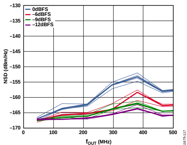
Figure 17. Single-Tone NSD vs. f_{OUT} over Digital Back Off, f_{DAC} = 1966 \text{ MHz}
