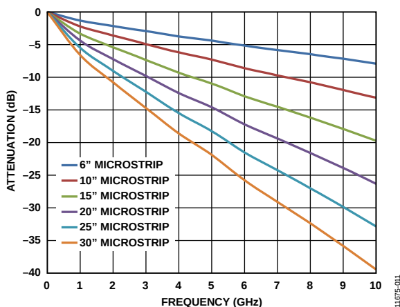
Figure 41. Insertion Loss of 50 \Omega Microstrips on FR4
