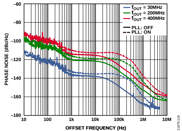
Figure 19. Single-Tone Phase Noise vs. Offset Frequency over f_{OUT} , f_{DAC} = 2.0 \text{ GHz} , PLL On and Off
