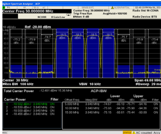
Figure 22. 4C WCDMA ACLR, f_{OUT} = 30 MHz, f_{DAC} = 983 MHz, 2× Interpolation, PLL Frequency = 122 MHz
