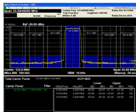
Figure 21. 1C WCDMA ACLR, f_{OUT} = 122 \text{ MHz} , f_{DAC} = 983 \text{ MHz} , 2× Interpolation, PLL Frequency = 122 MHz
