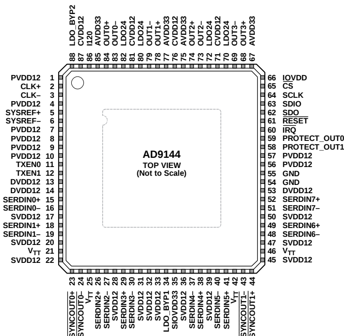
Figure 3. Pin Configuration
