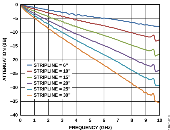
Figure 40. Insertion Loss of 50 \Omega Striplines on FR4
