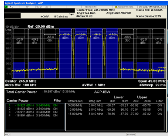
Figure 25. 4C WCDMA ACLR, f_{OUT} = 245 MHz, f_{DAC} = 1966 MHz, 4× Interpolation, PLL Frequency = 245 MHz
