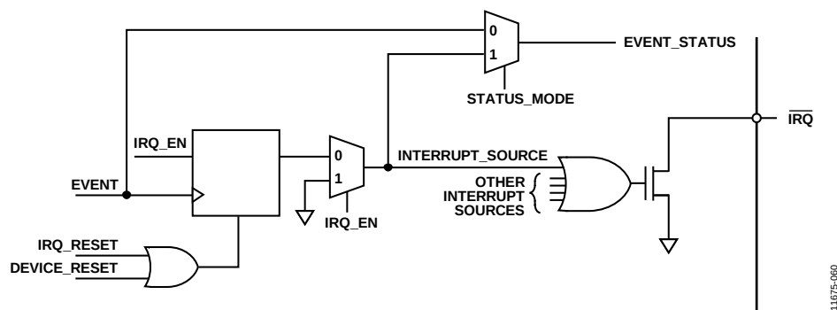
Figure 75. Simplified Schematic of IRQ Circuitry
