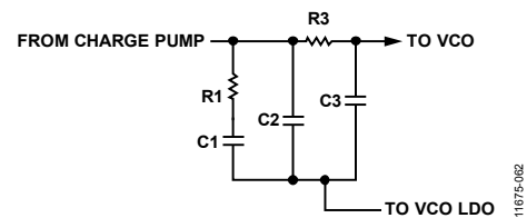
Figure 77. Loop Filter
