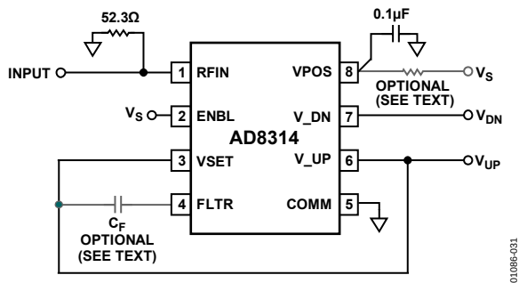
Figure 31. Basic Connections for Operation in Measurement Mode
