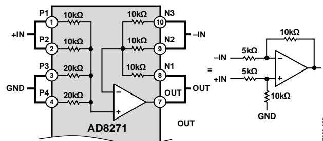
Figure 47. Gain = 2 Difference Amplifier, Referenced to Ground
