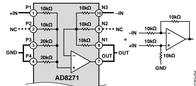
Figure 46. Gain = 1 Difference Amplifier, Referenced to Ground
