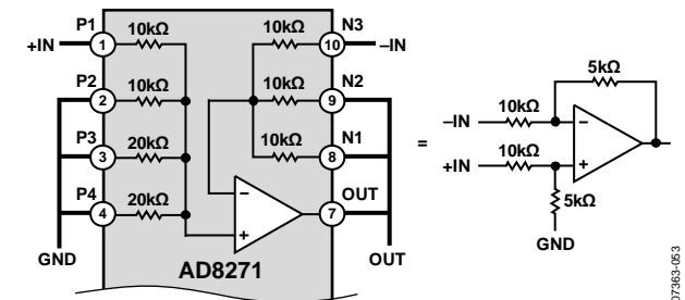
Figure 45. Gain = 1/2 Difference Amplifier, Referenced to Ground
