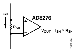
Figure 51. AD8276 Monitoring Current Through a Shunt Resistor
