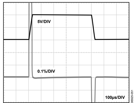
Figure 25. Large Signal Response, G = 5
