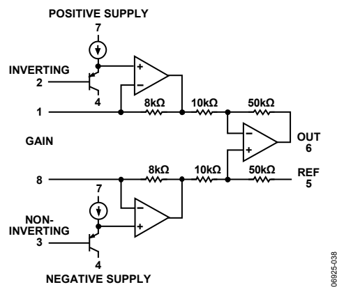
Figure 31. Simplified Schematic
