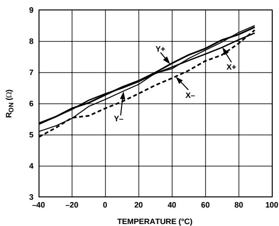
Figure 14. Switch-On Resistance vs. Temperature (X+, Y+: +VCC to Pin; X-, Y-: Pin to GND)
