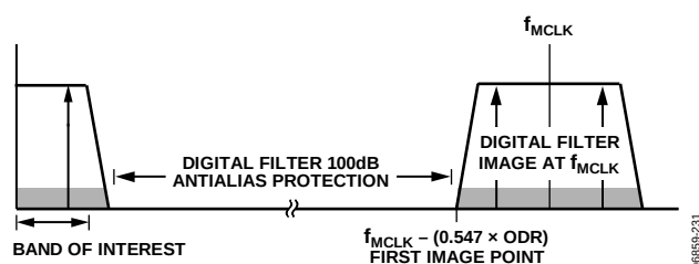
Figure 42. AD7767/AD7767-1/AD7767-2 Spectrum
