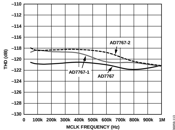
Figure 19. AD7767/AD7767-1/AD7767-2 THD vs. MCLK Frequency
