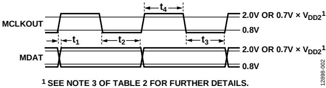
Figure 2. Data Timing
