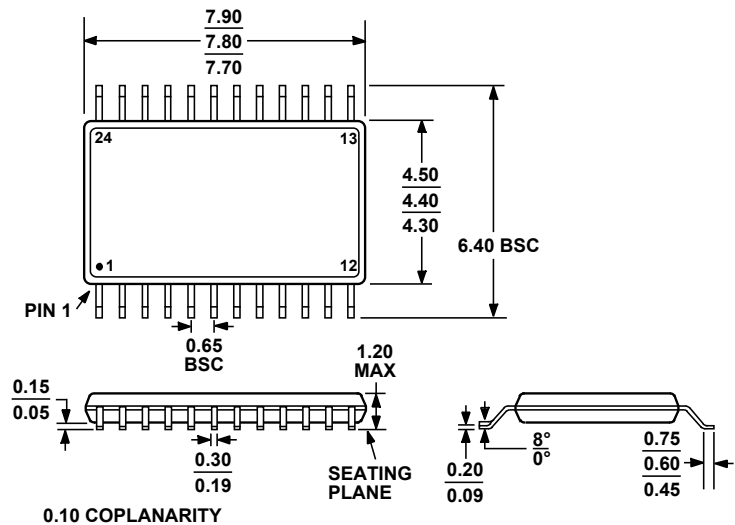
COMPLIANT TO JEDEC STANDARDS MO-153-AD Figure 33. 24-Lead Thin Shrink Small Outline Package [TSSOP] (RU-24) Dimensions shown in millimeters
