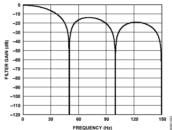
Figure 64. Filter Response for Average + Decimate Filter (Sinc 3 Filter, FS[9:0] = 6 , Average by 16)
