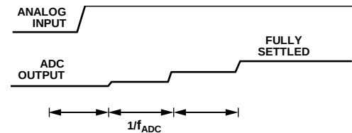
Figure 51. Asynchronous Step Change in Analog Input (Sinc 3 Chop Enabled)
