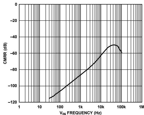
Figure 16. Common-Mode Rejection Ratio (CMRR) vs. V_{IN} Frequency ( V_{IN} = 0.1\text{ V} )
