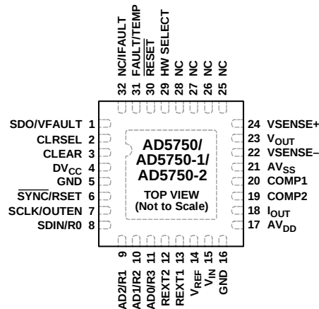
Figure 4. Pin Configuration
