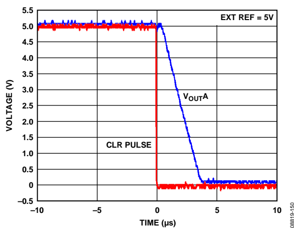
Figure 44. Hardware \overline{\text{CLR}}
