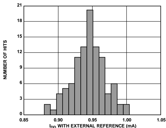
Figure 22. I_{DD} Histogram with External Reference
