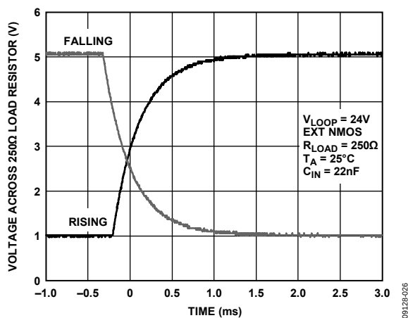
Figure 27. Full-Scale Loop Current Step, C IN = 22 nF
