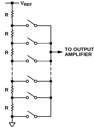
Figure 37. Resistor String
