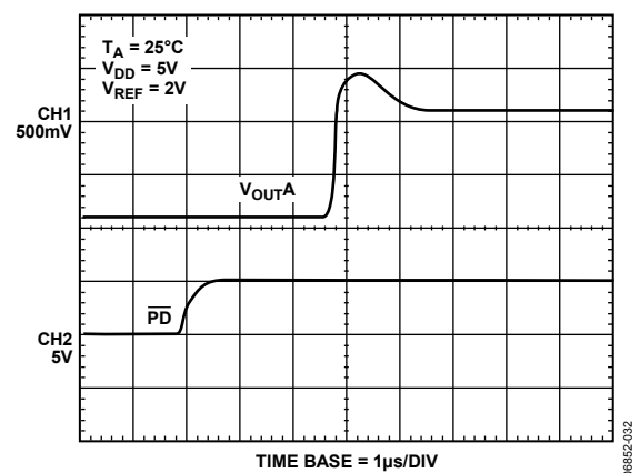
Figure 31. Exiting Power-Down to Midscale
