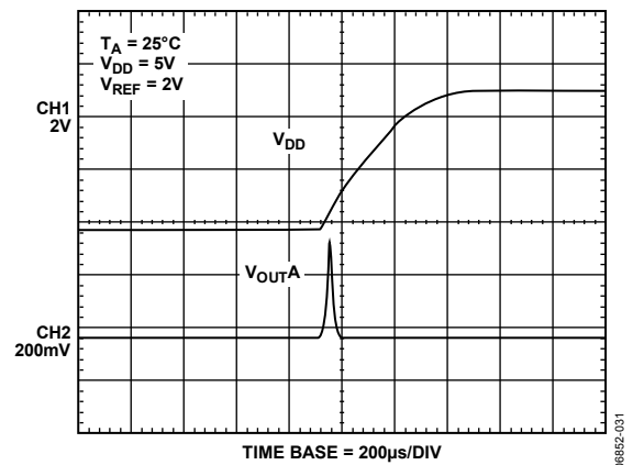
Figure 30. Power-On Reset to 0 V
