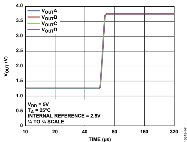
Figure 29. Settling Time
