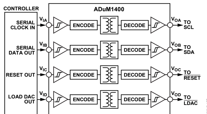
Figure 51. Isolated Interface
