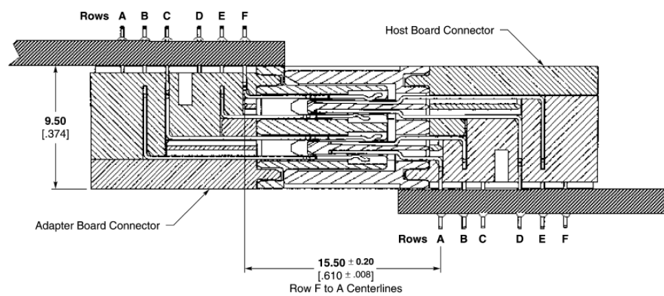
Inverted Application
