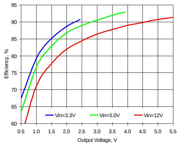
Figure 5. Efficiency vs. Output Voltage, Iout=10A, Fsw=500kHz
