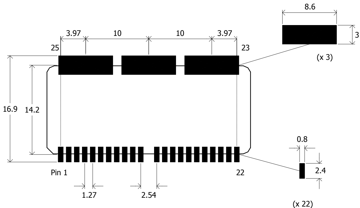
Figure 58. Recommended Pad Sizes
