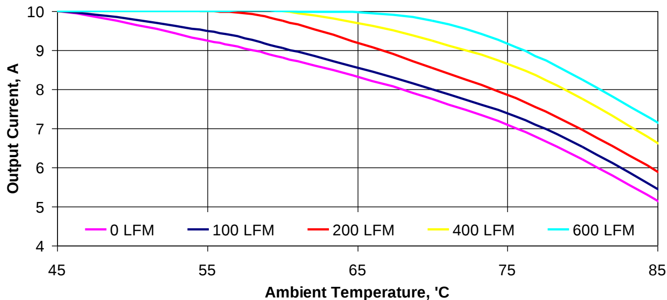
Figure 24. Thermal Derating Curves. Vin=13.2V, Vout=5.0V, Fsw=1MHz
