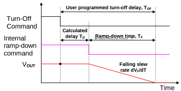
Figure 35. Relationship between Turn-Off Delay and Falling Slew Rate
