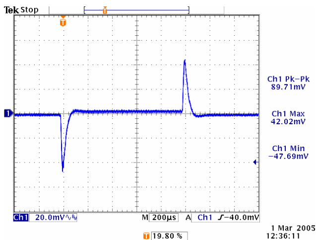
Figure 19. Vin=12V, Vout=1V, BW=60kHz.
