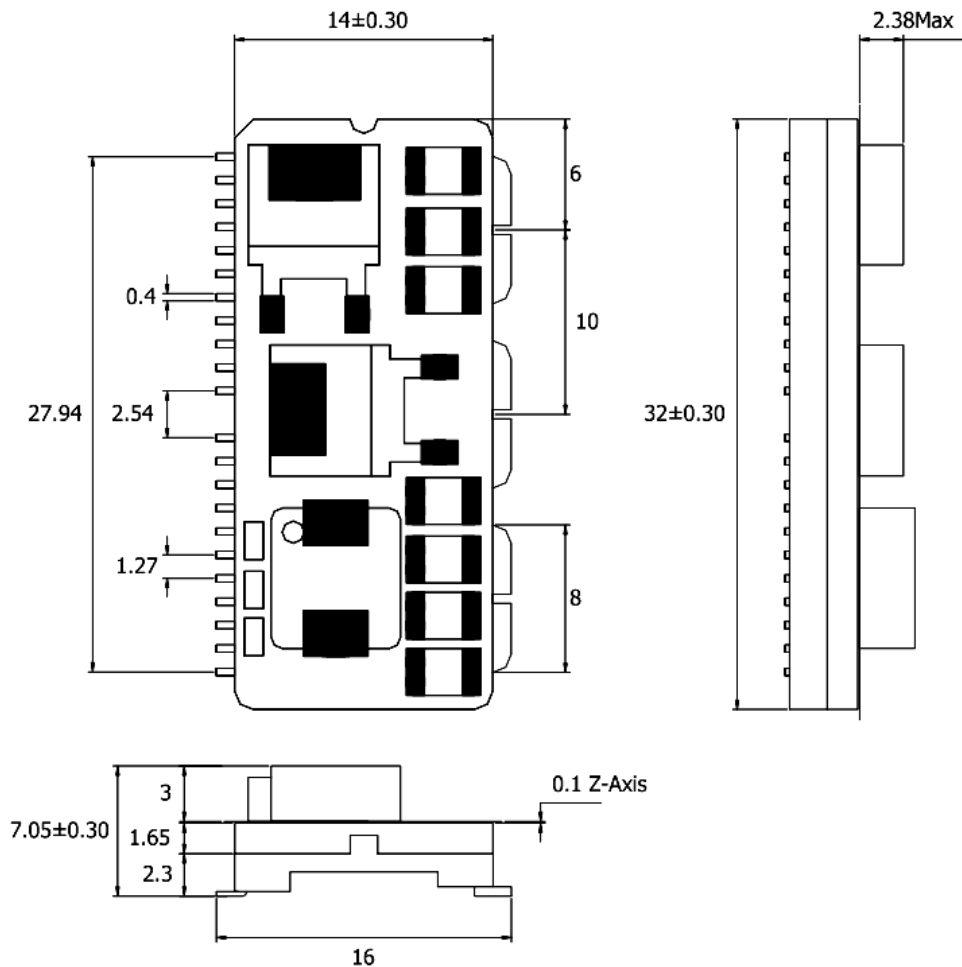
Figure 57. Mechanical Drawing
