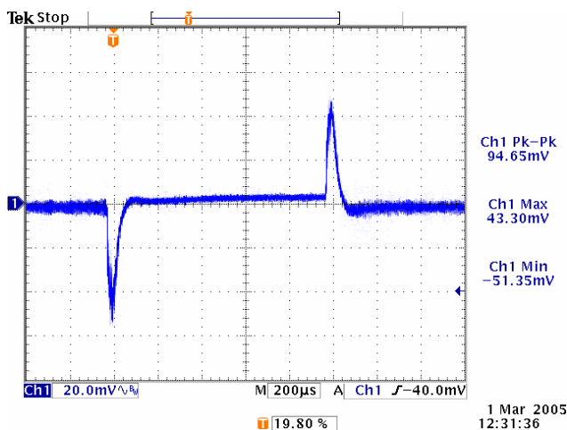
Figure 18. Vin=12V, Vout=5V, BW=60kHz.
