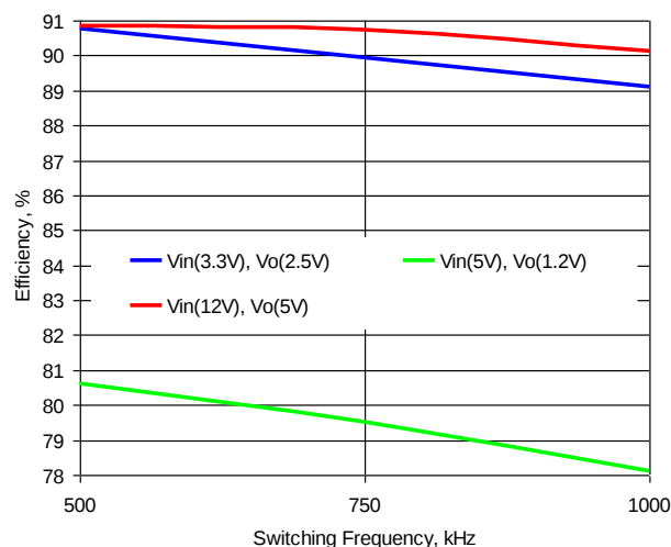
Figure 10. Efficiency vs. Switching Frequency. I_{out}=10A
