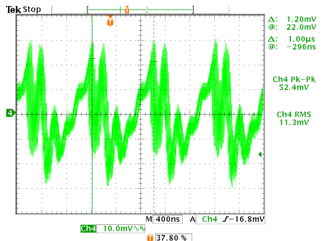
Figure 49. Input Voltage Noise, No Interleave
