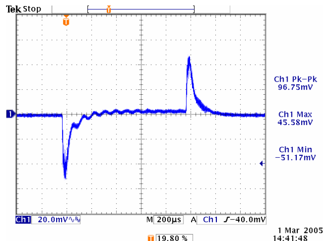
Figure 20. Vin=5V, Vout=2.5V, BW=60kHz.
