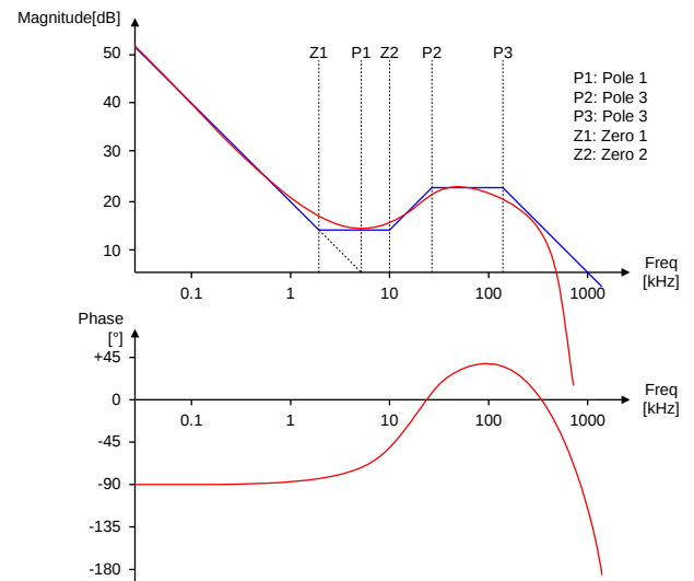
Figure 54. Transfer Function of PWM
