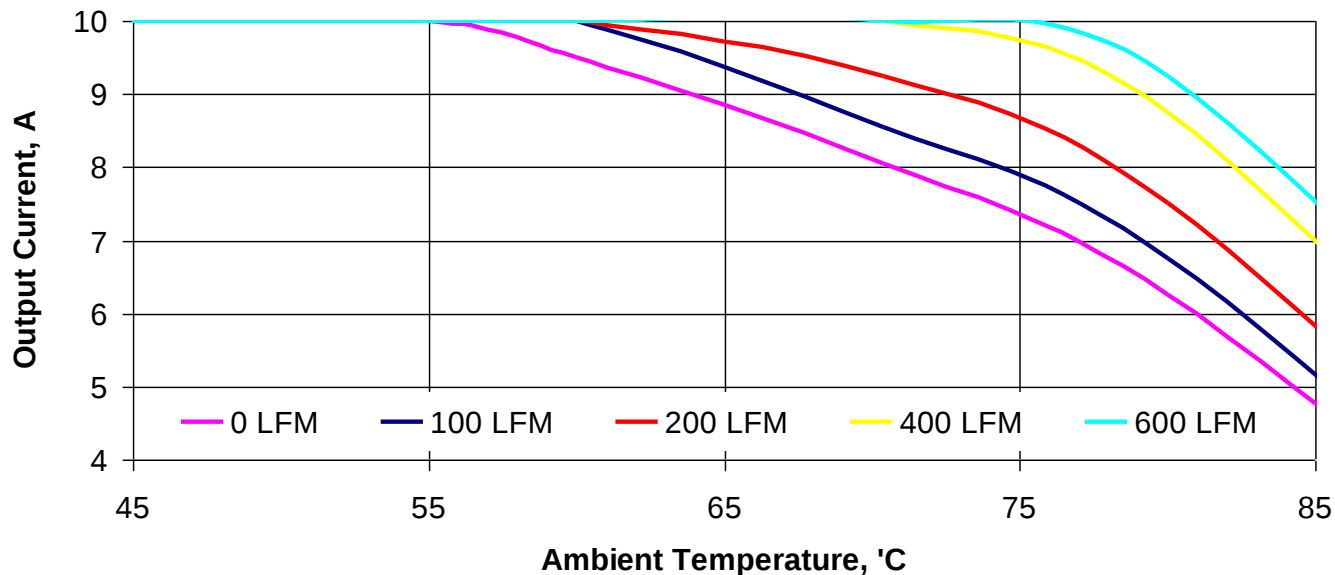
Figure 23. Thermal Derating Curves. Vin=13.2V, Vout=5.0V, Fsw=500kHz
