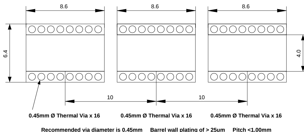
Figure 59. Recommended PCB Layout for Multilayer PCBs
