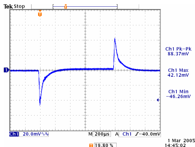
Figure 21. Vin=5V, Vout=1V, BW=60kHz.
