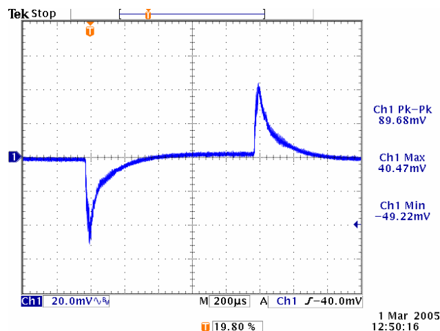
Figure 22. Vin=3.3V, Vout=1V, BW=60kHz.
