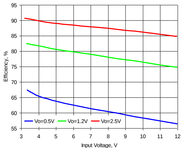
Figure 6. Efficiency vs. Input Voltage. Iout=10A, Fsw=500kHz
