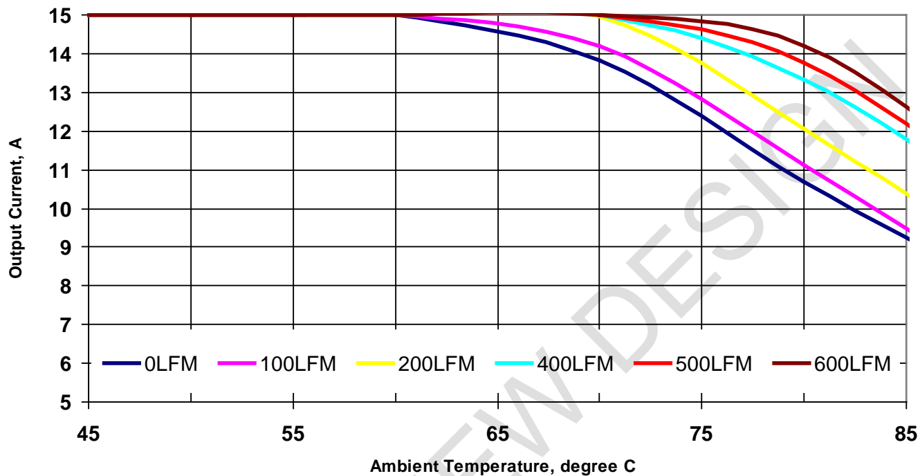
Figure 15. Thermal Derating Curves. Vin=12V, Vout=5.0V
