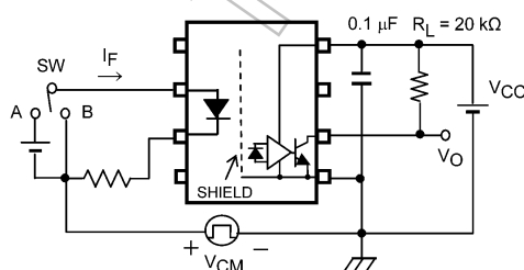
Fig. 12.1.7 Common-Mode Transient Immunity and waveform
