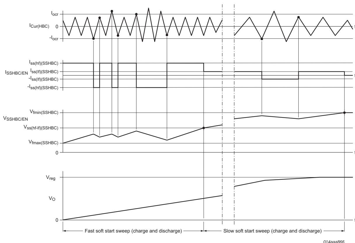
Fig 16. Overcurrent regulation during start-up
