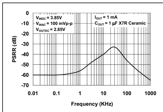
FIGURE 2-18: Power Supply Rejection Ratio vs. Frequency.
