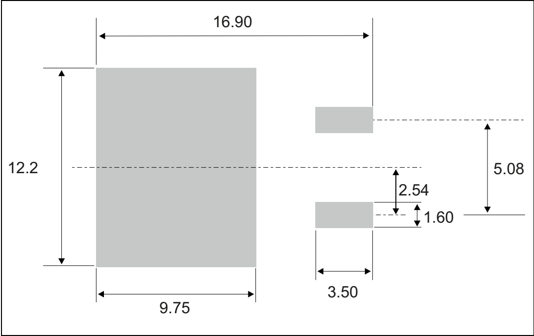
Figure 18. D 2 PAK footprint (dimensions in mm)
