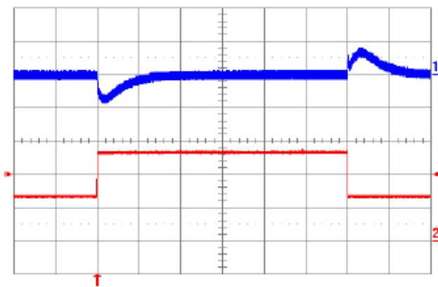
Fig. 8.0V.12: Output voltage response to load current step-change (1.325A – 2.65A – 1.325A) at V_{in} = 48V . Top trace: output voltage (200 mV/div.). Bottom trace: load current (1 A/div.). Current slew rate: 5 A/ \mu s. C_o = 94 \mu F tantalum + 1 \mu F ceramic. Time scale: 0.5 ms/div.
