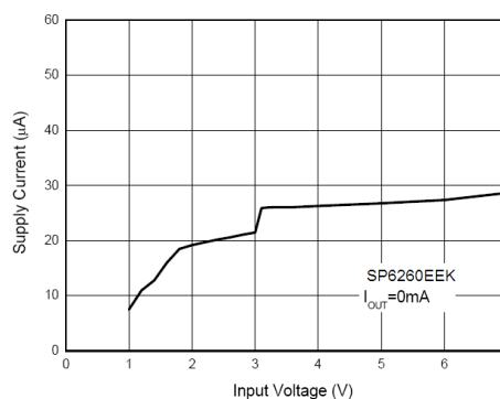
Fig. 16: Supply Current vs. Input Voltage SP6260EEK (3.0V)
