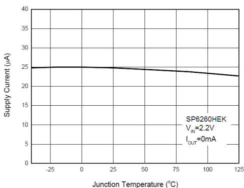
Fig. 17: Supply Current vs. Junction Temperature SP6260HEK (1.2V)
