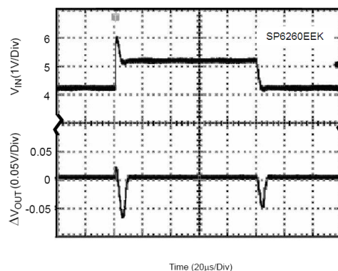
Fig. 20: Line Transient SP6260EEK (3.0V) (Conditions: I_{OUT}=30\text{mA} , C_{IN}=1\mu\text{F} , C_{OUT}=1\mu\text{F} )
