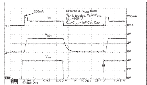
In-Rush Current ( V_{IN} = 4V , I_{OUT} = 100\mu A )
