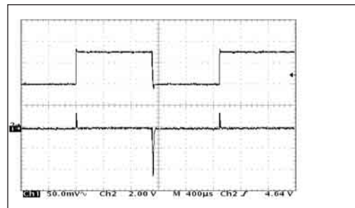
Line Transient Response ( V_{IN}=7V , I_{OUT}=10\mu A )
