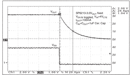
Turn off Time ( V_{IN} = 4V , I_{OUT} = 100\mu A )
