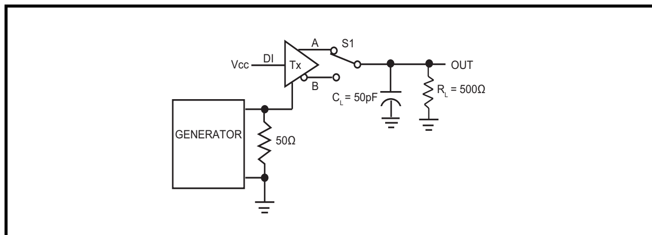
FIGURE 8. RS-485 DRIVER ENABLE AND DISABLE TIMING DIAGRAM
