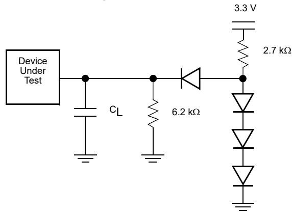
Figure 13. Test Setup
