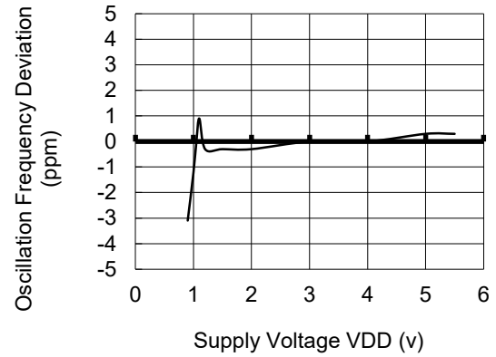
Oscillation Frequency Deviation vs. Supply Voltage (T opt =25°C, VDD=3V as standard)
