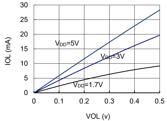
V OL vs. I OL (SDA pin, T opt =25°C)
