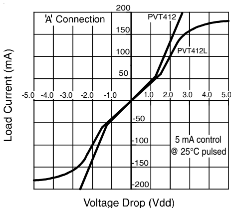
Figure 3. Linearity Characteristics
