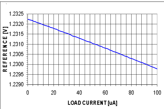
Figure 11. Voltage reference vs load current
