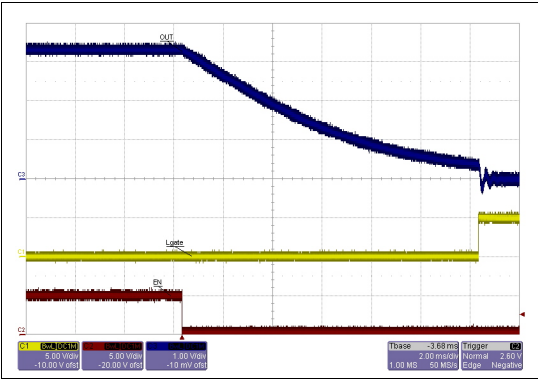
Figure 26. OUT1 = 3.3 V soft-end (0.8 \Omega load)
