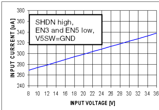
Figure 10. Standby mode input battery current vs input voltage
