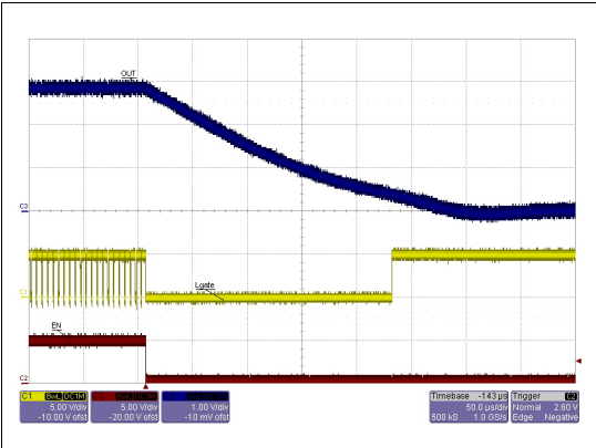
Figure 26. OUT1 = 3.3 V soft-end (0.8 \Omega load)
