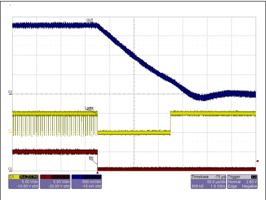
Figure 27. OUT2 = 1.8 V soft-end (0.6 \Omega load)
