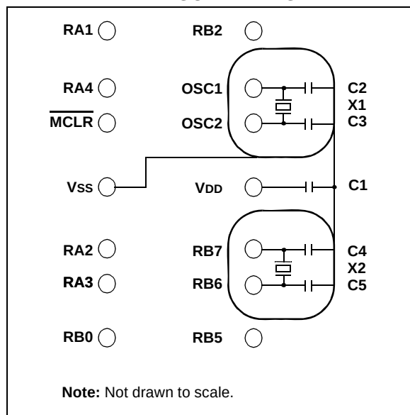
FIGURE 12-4: OSCILLATOR CIRCUIT WITH GROUNDED GUARD RING
