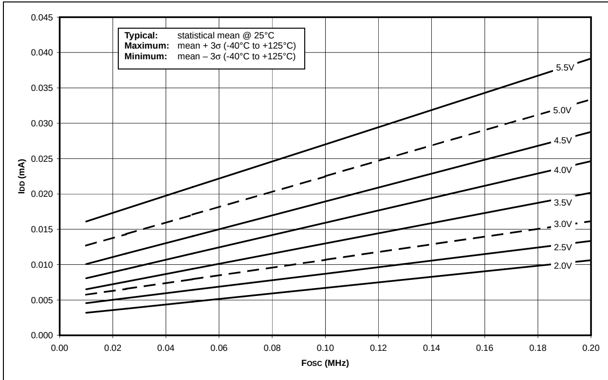
FIGURE 23-9: MAXIMUM I_{DD} vs. F_{osc} OVER V_{DD} PRI_IDLE, EC MODE, -40^{\circ}\text{C} TO +85^{\circ}\text{C}
