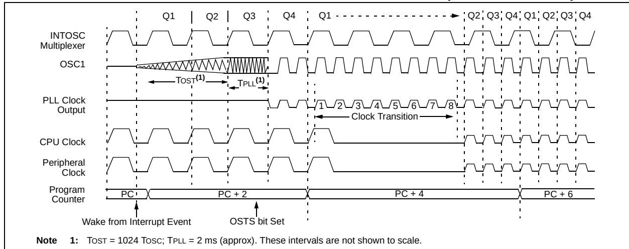
FIGURE 19-2: TIMING TRANSITION FOR TWO-SPEED START-UP (INTOSC TO HSPLL)
