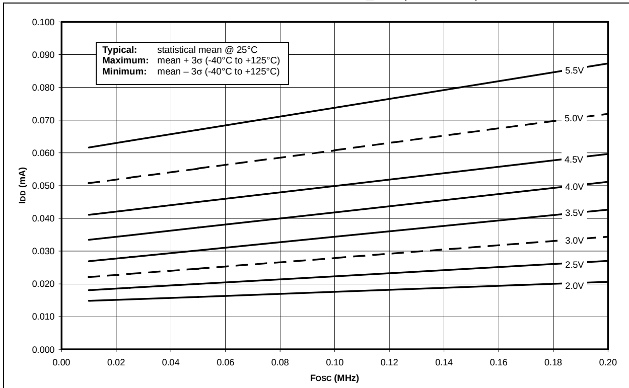
FIGURE 23-10: MAXIMUM I_{DD} vs. F_{osc} OVER V_{DD} PRI_IDLE, EC MODE, -40^{\circ}\text{C} TO +125^{\circ}\text{C}
