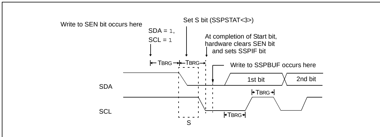
FIGURE 10-19: FIRST START BIT TIMING
