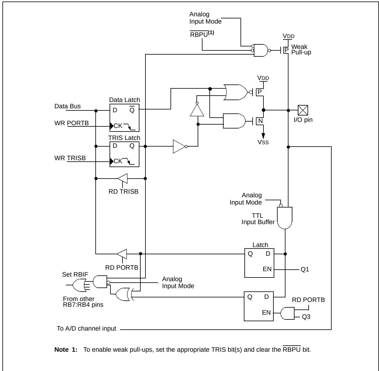
FIGURE 5-12: BLOCK DIAGRAM OF RB4/AN11 PIN
