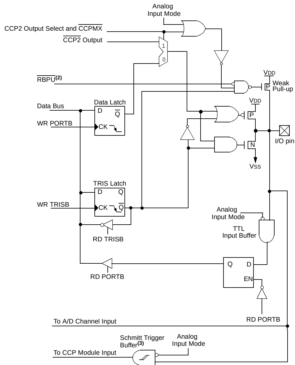
FIGURE 5-11: BLOCK DIAGRAM OF RB3/CCP2 (1) /AN9 PIN
