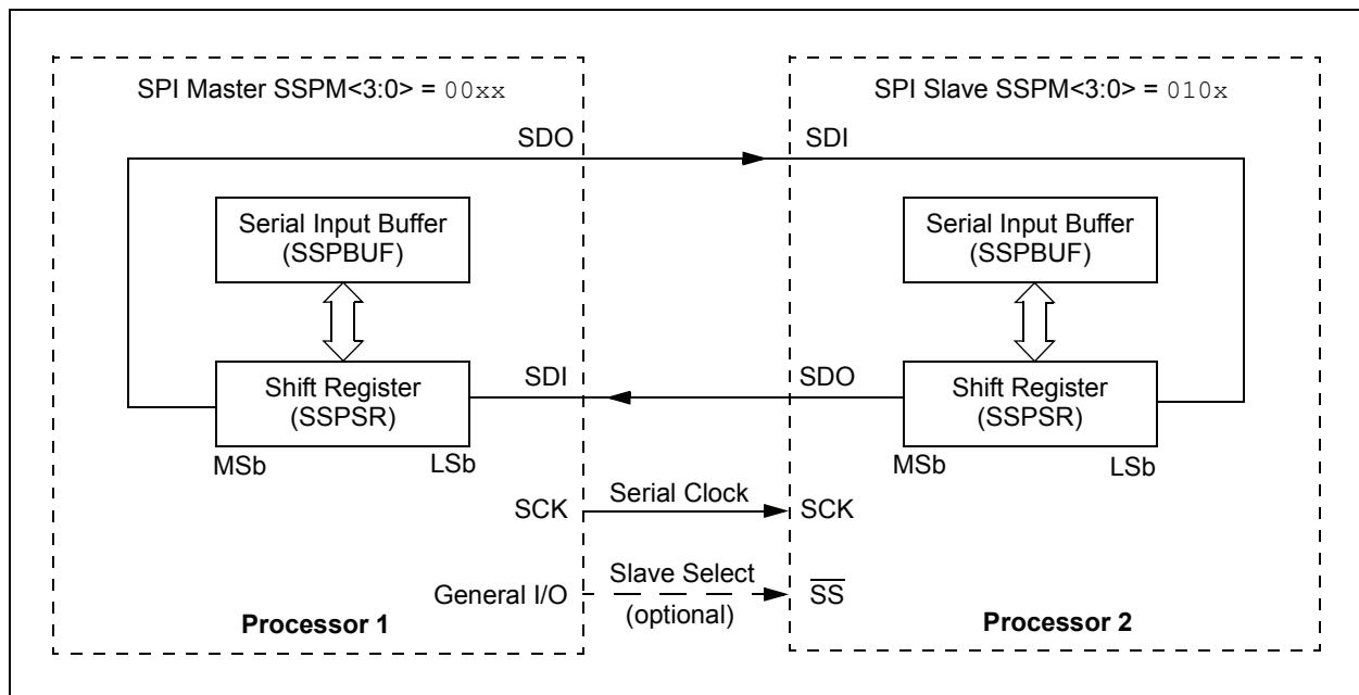
FIGURE 17-1: TYPICAL SPI MASTER/S�AVE CONNECTION
