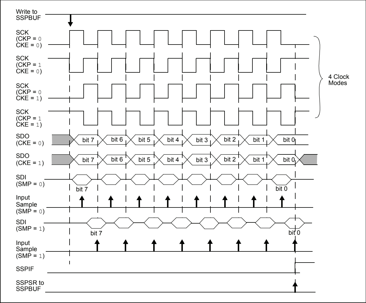
EXAMPLE 17-1: LOADING THE SSPBUF (SSPSR) REGISTER
