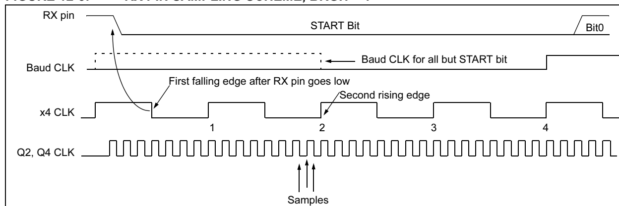
FIGURE 12-3: RX PIN SAMPLING SCHEME, BRGH = 1
