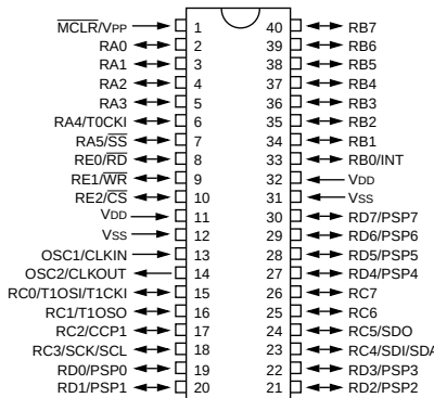
PIC16C64
