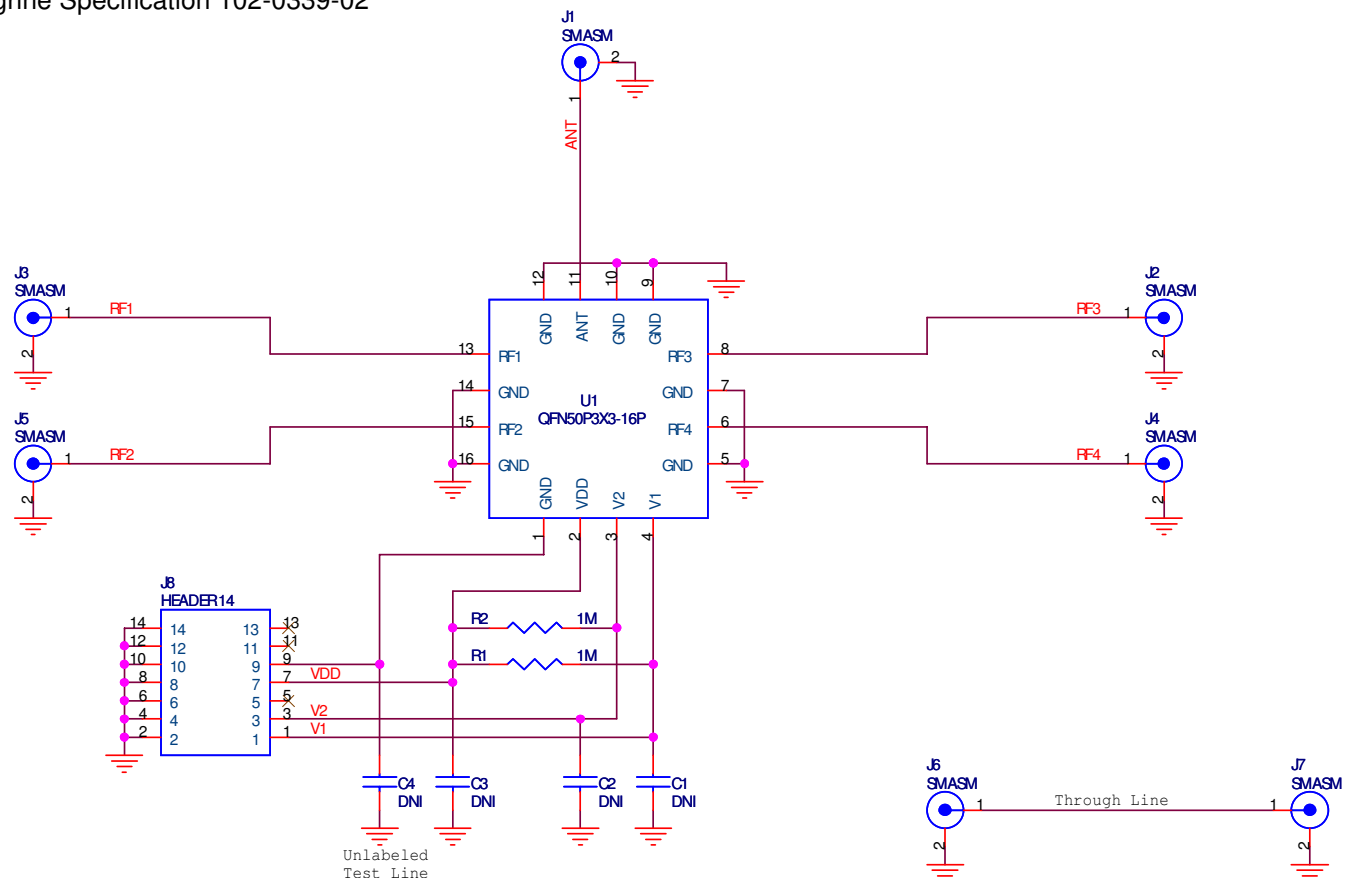
Figure 5. Evaluation Board Schematic Peregrine Specification 102-0339-02
