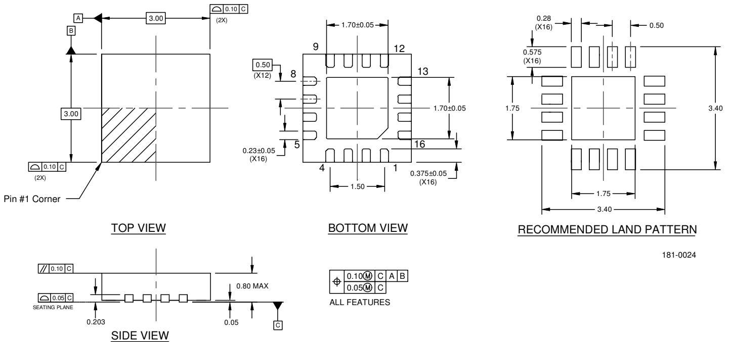
Figure 13. Package Drawing
