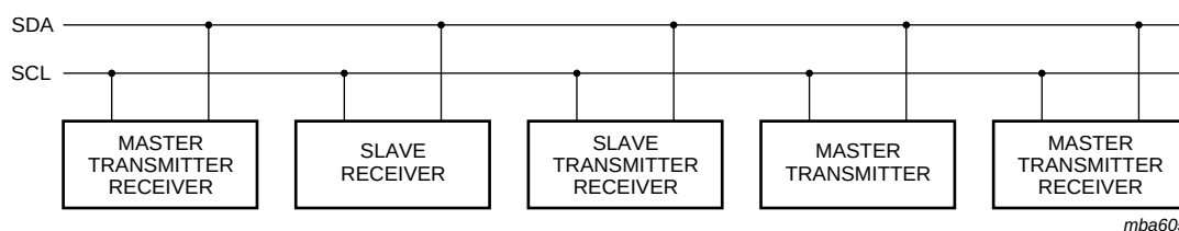
Fig 40. System configuration
