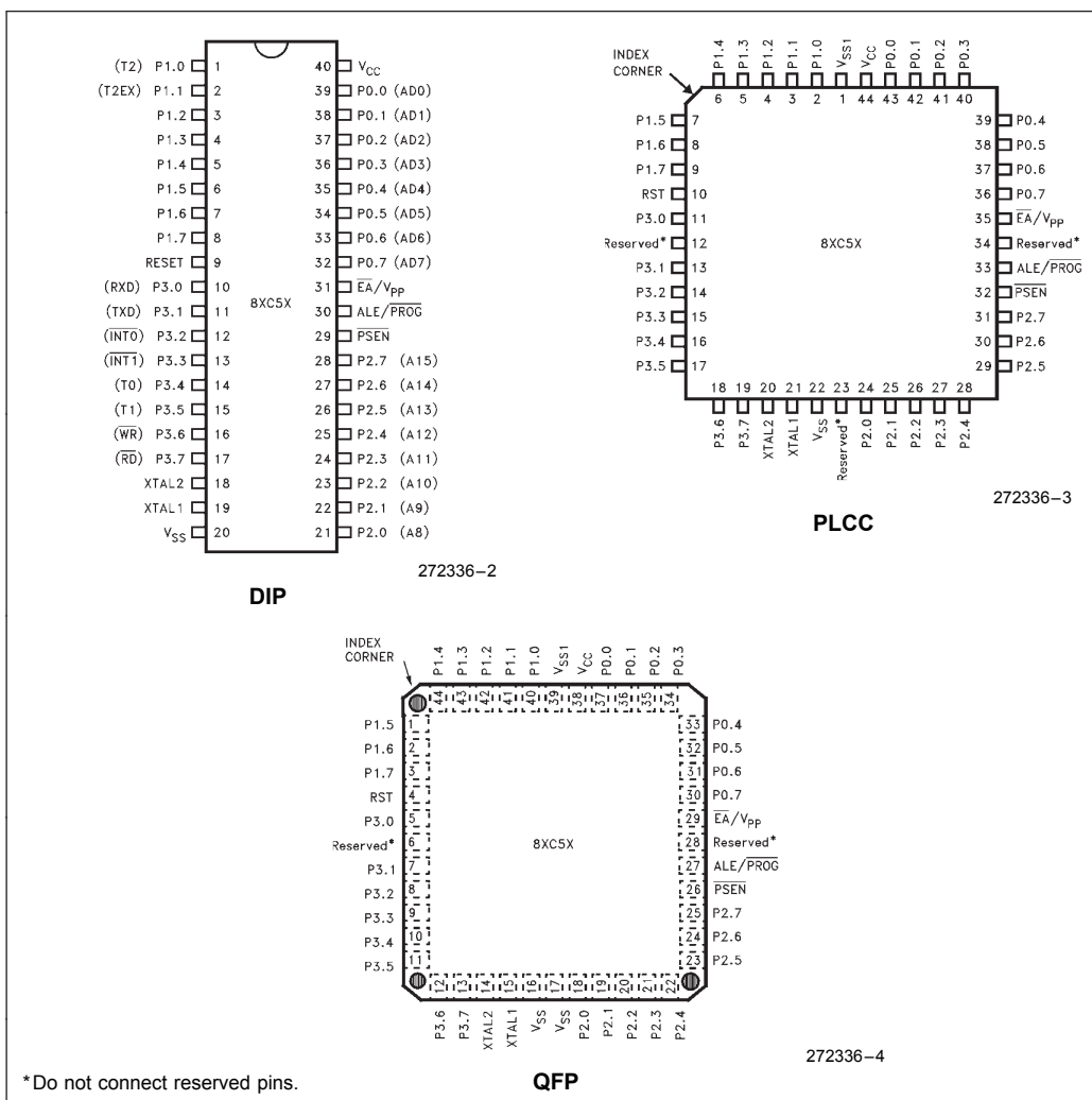
Figure 2. Pin Connections
