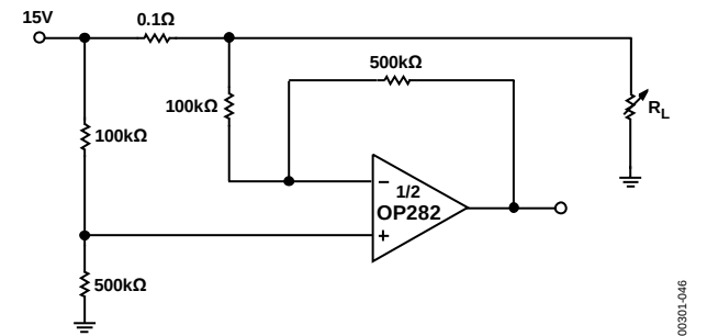
Figure 45. High-Side Signal Conditioning
