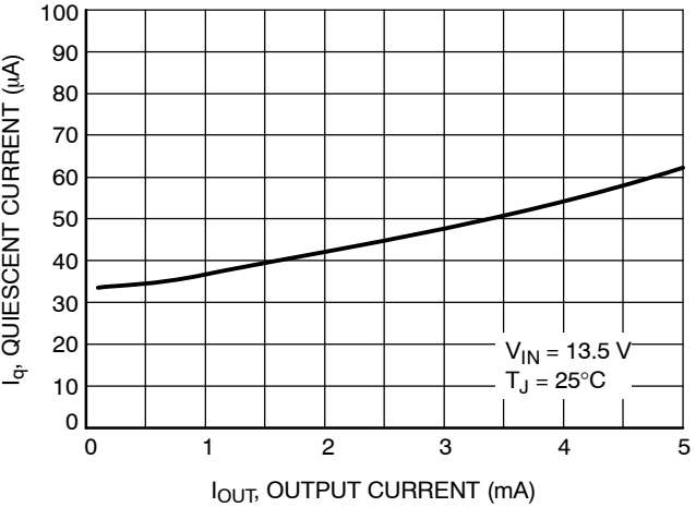
Figure 17. Quiescent Current vs. Output Current (3.3 V Version) (Low Load)
