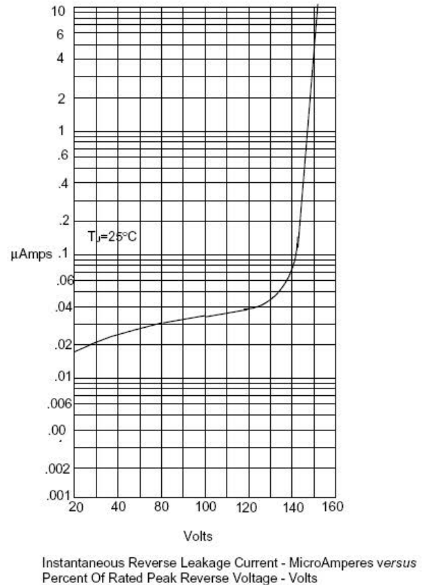
Figure 2. Typical Reverse Current
