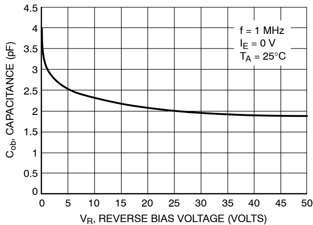
Figure 34. Output Capacitance
