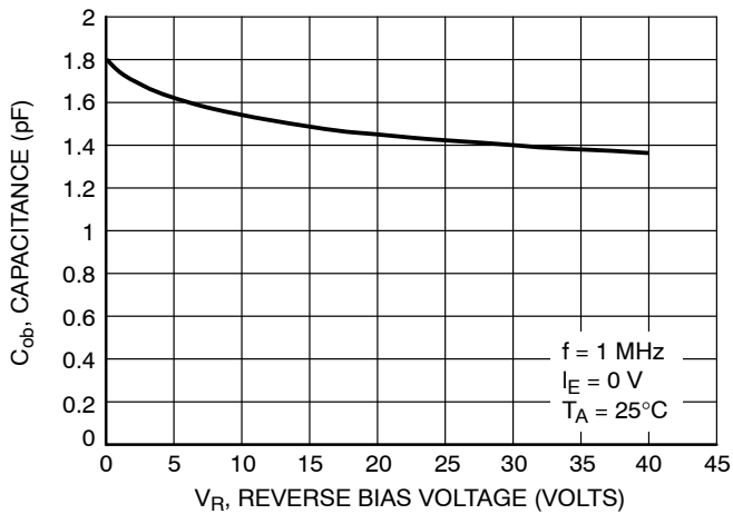
Figure 54. Output Capacitance
