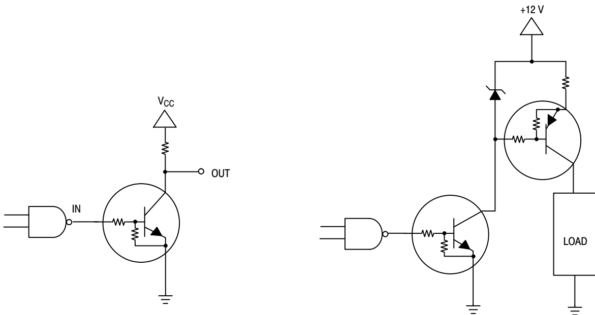
Figure 58. Open Collector Inverter: Inverts the Input Signal
