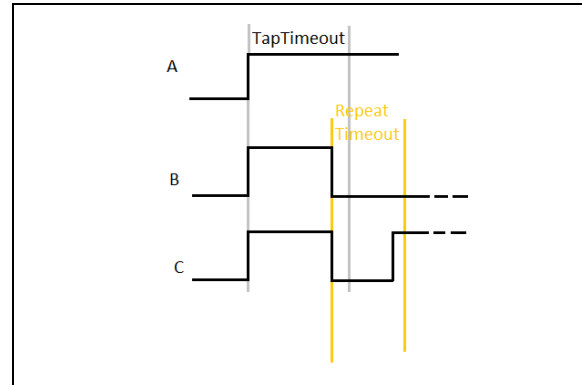
FIGURE 11-3: TAP RECOGNIZER
