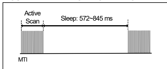
FIGURE 4-2: LOW-POWER MODE
