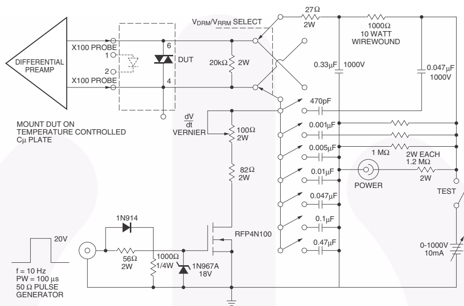
Figure 11. Circuit for Static dv/dt Measurement of Power Thyristors
