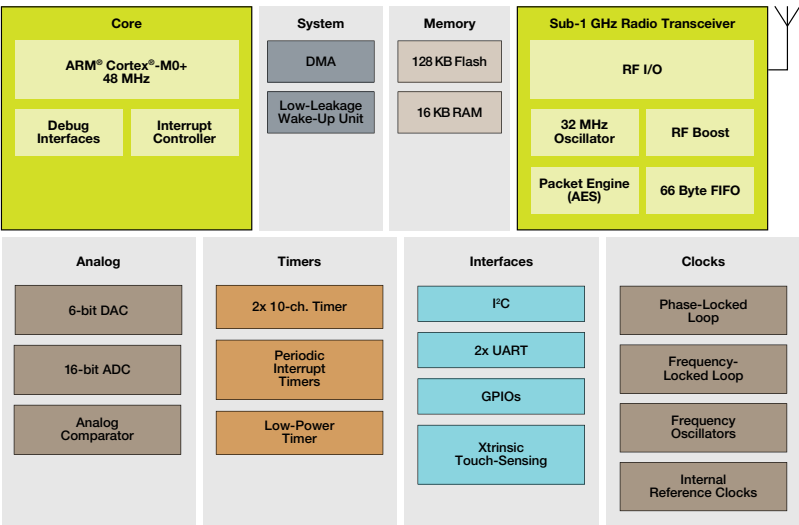
Kinetis KW0x Wireless MCU Block Diagram
